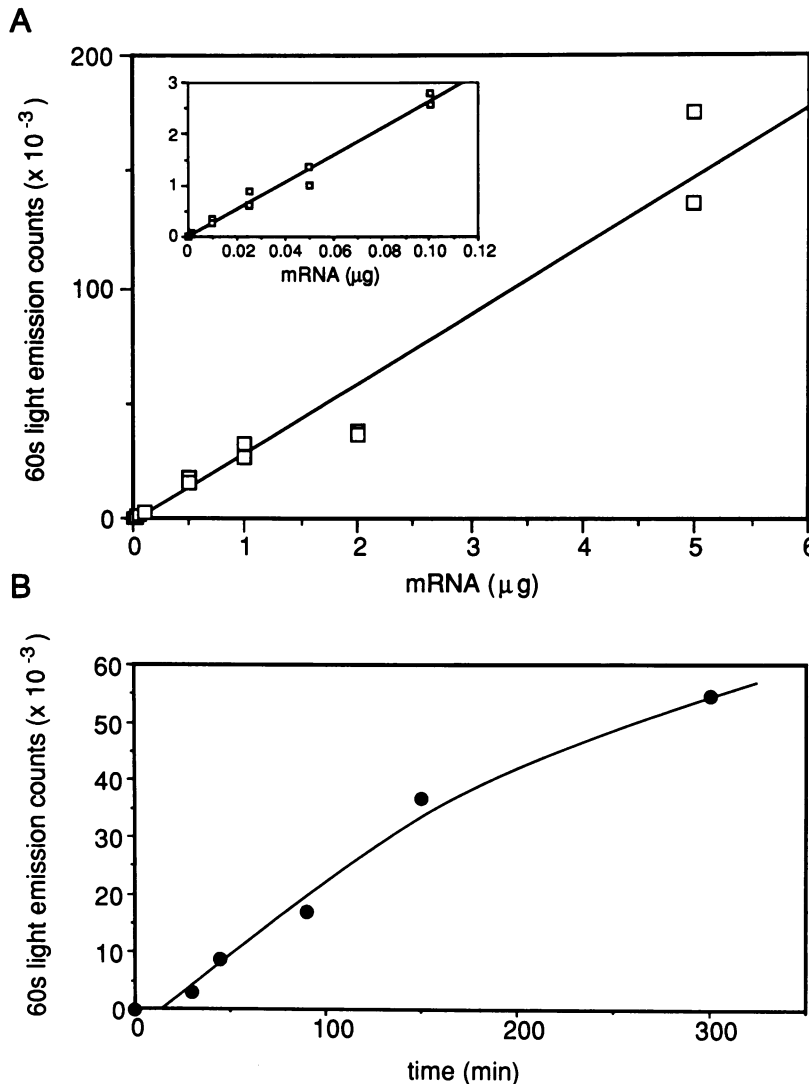
FIG. 3. Kinetics of mRNA transfection. (A) Subconfluent 10-cm dishes of NIH 3T3 cells were transfected with various quantities of mRNA (Cap-βg Luc βg An) with the addition of carrier RNA to a total of 20 µg per transfection under the standard conditions. Lysates were prepared 8 hr after addition of RNA/lipofectin complex to cells and analyzed for luciferase specific activity as described. (Inset) Data near the origin shown with expanded scales. All transfections were performed in duplicate as shown. (B) Transfections were performed as above with 5 µg of mRNA and no carrier. Addition of nonspecific RNA increases the overall luciferase protein production (about 2-fold), presumably by altering stability of mRNA (6). Lysates were prepared at the time indicated and then analyzed for luciferase specific activity.
